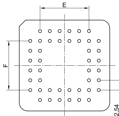
PCB LAYOUT
