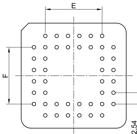
PCB LAYOUT
